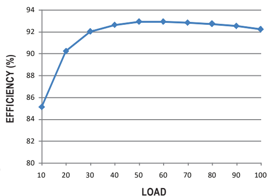
The curve above is measured at 230VAC.
